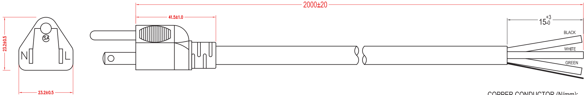
Plug type
